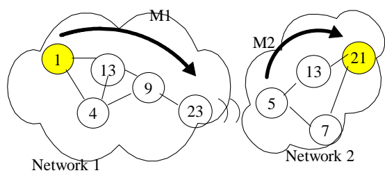
Fig. 2. Merging Networks
