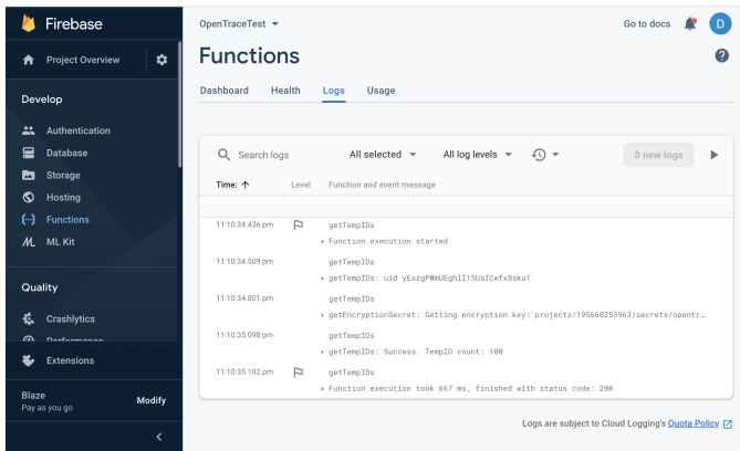
Fig. 1. Example of Firebase Functions logging visible to the operator of the OpenTrace app. Observe that there is fine-grained logging of individual function calls per user (the uid value in these logs is a unique identifier linked to a users phone number). The tempIDs function is, for example, regularly called by the OpenTrace app to refresh the set of tempIDs available for a mobile handset to advertise on Bluetooth.
